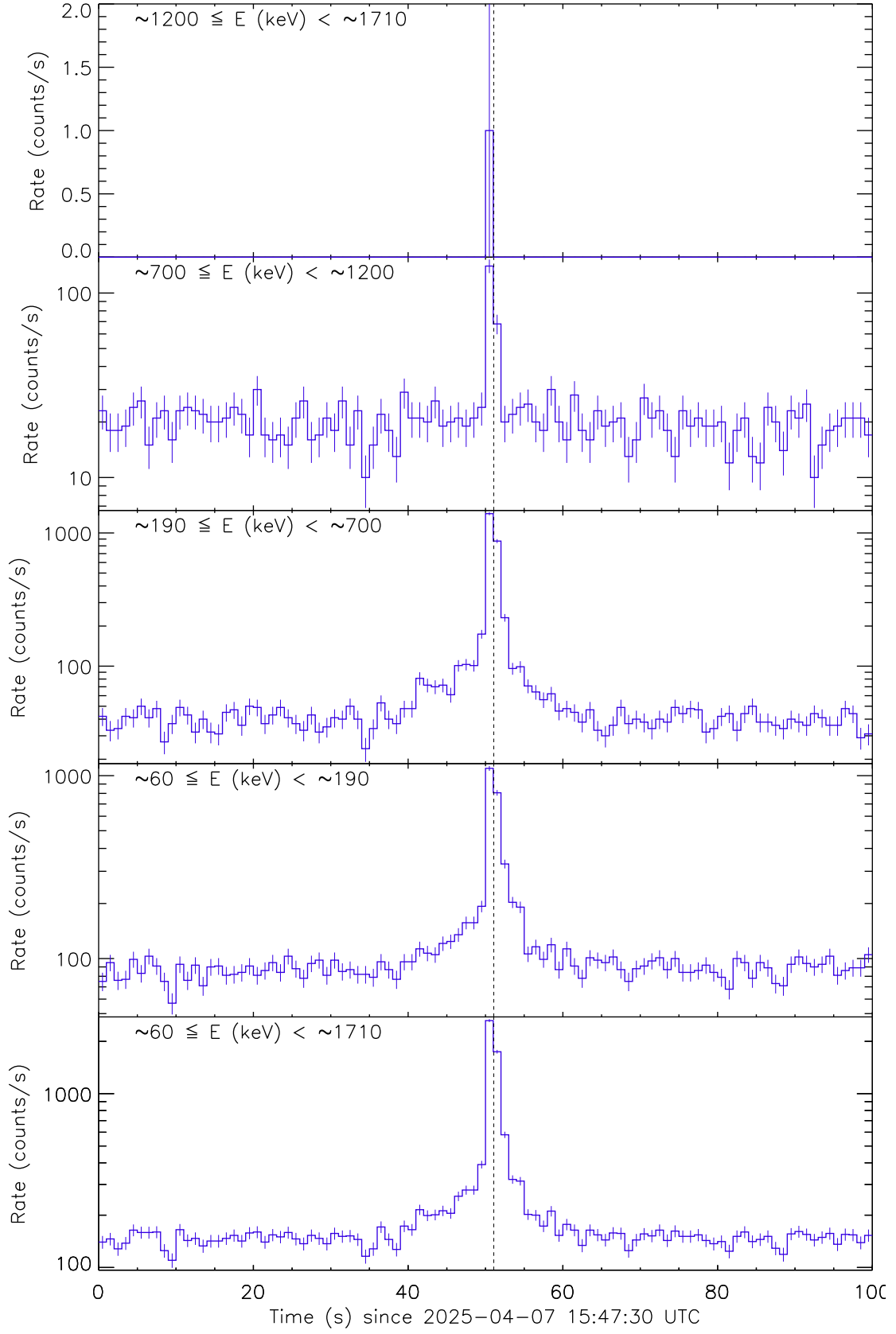
Figure 4: Raw count rate curves of GRB 250407A recorded by the detector unit no. 1. The vertical dashed line marks the trigger time by Fermi/GBM.
