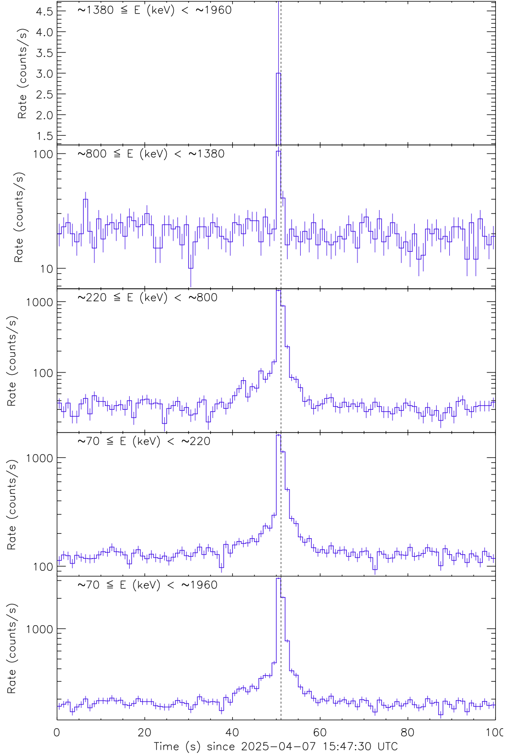
Figure 1: Raw count rate curves of GRB 250407A recorded by the detector unit no. 0. The vertical dashed line marks the trigger time by Fermi/GBM.
