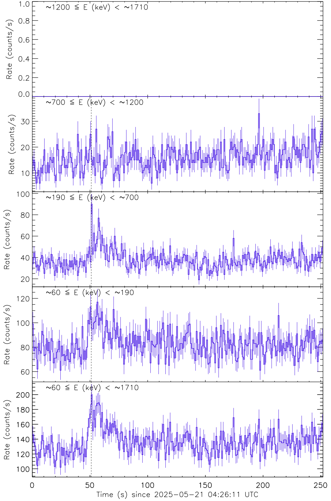
Figure 4: Raw count rate curves of GRB 250521A recorded by the detector unit no. 1. The vertical dashed line marks the trigger time by Fermi/GBM.
