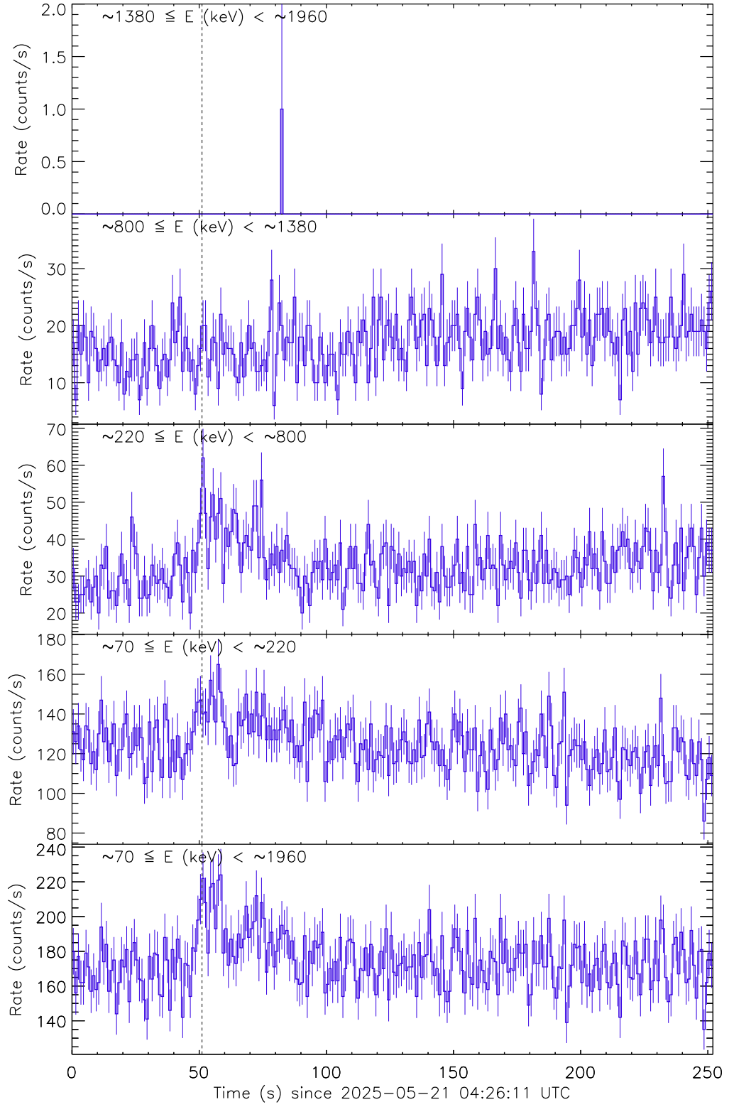
Figure 1: Raw count rate curves of GRB 250521A recorded by the detector unit no. 0. The vertical dashed line marks the trigger time by Fermi/GBM.
