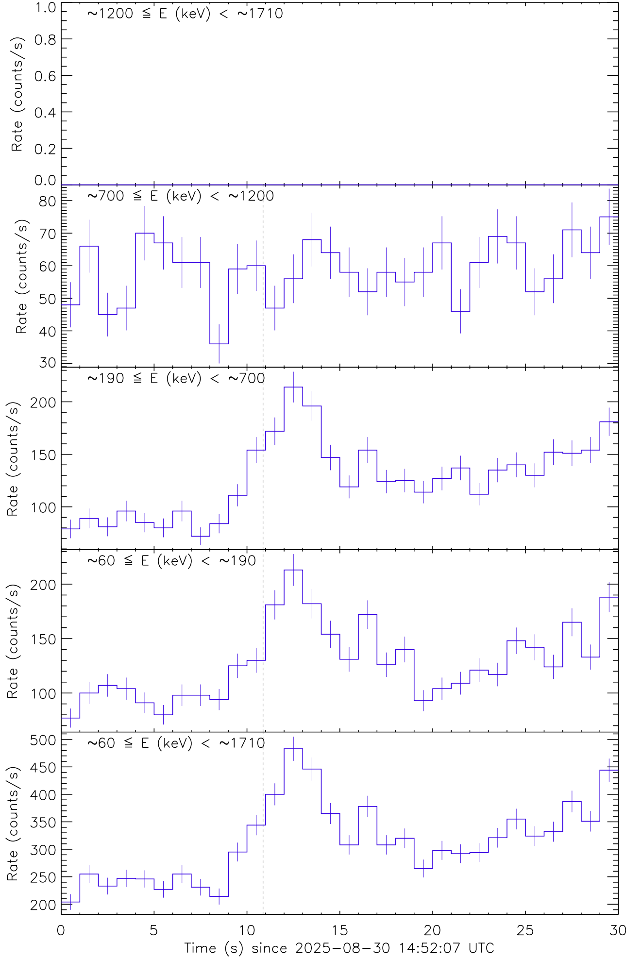
Figure 4: Raw count rate curves of GRB 250830C recorded by the detector unit no. 1. The vertical dashed line marks the trigger time by Konus-Wind.
