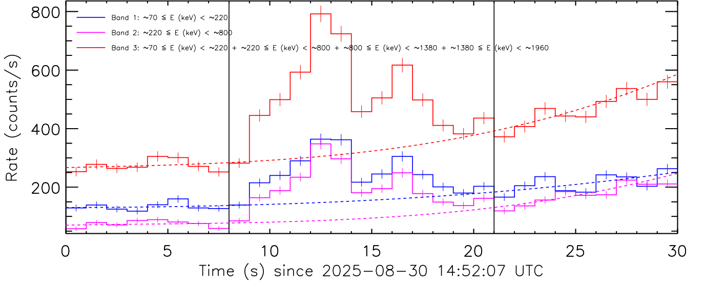
Figure 2: Background fit to the data from the detector unit no. 0 by a third order polynomial. Pre-burst and post-burst intervals which were used for the background fit are delimited by the vertical solid lines.
