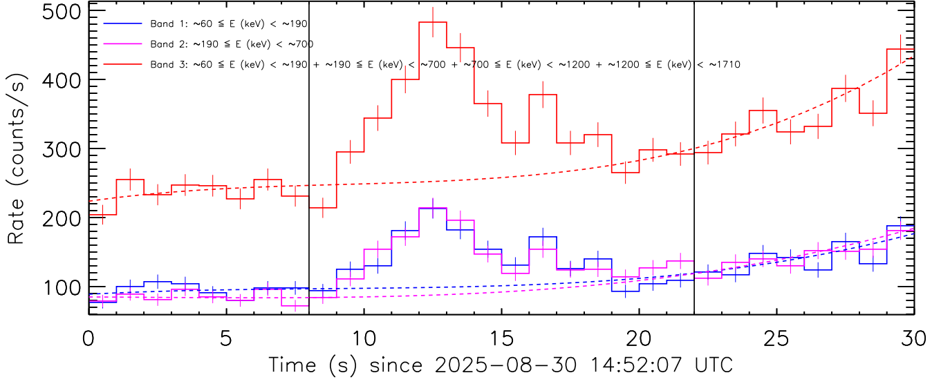
Figure 5: Background fit to the data from the detector unit no. 1 by a third order polynomial. Pre-burst and post-burst intervals which were used for the background fit are delimited by the vertical solid lines.
