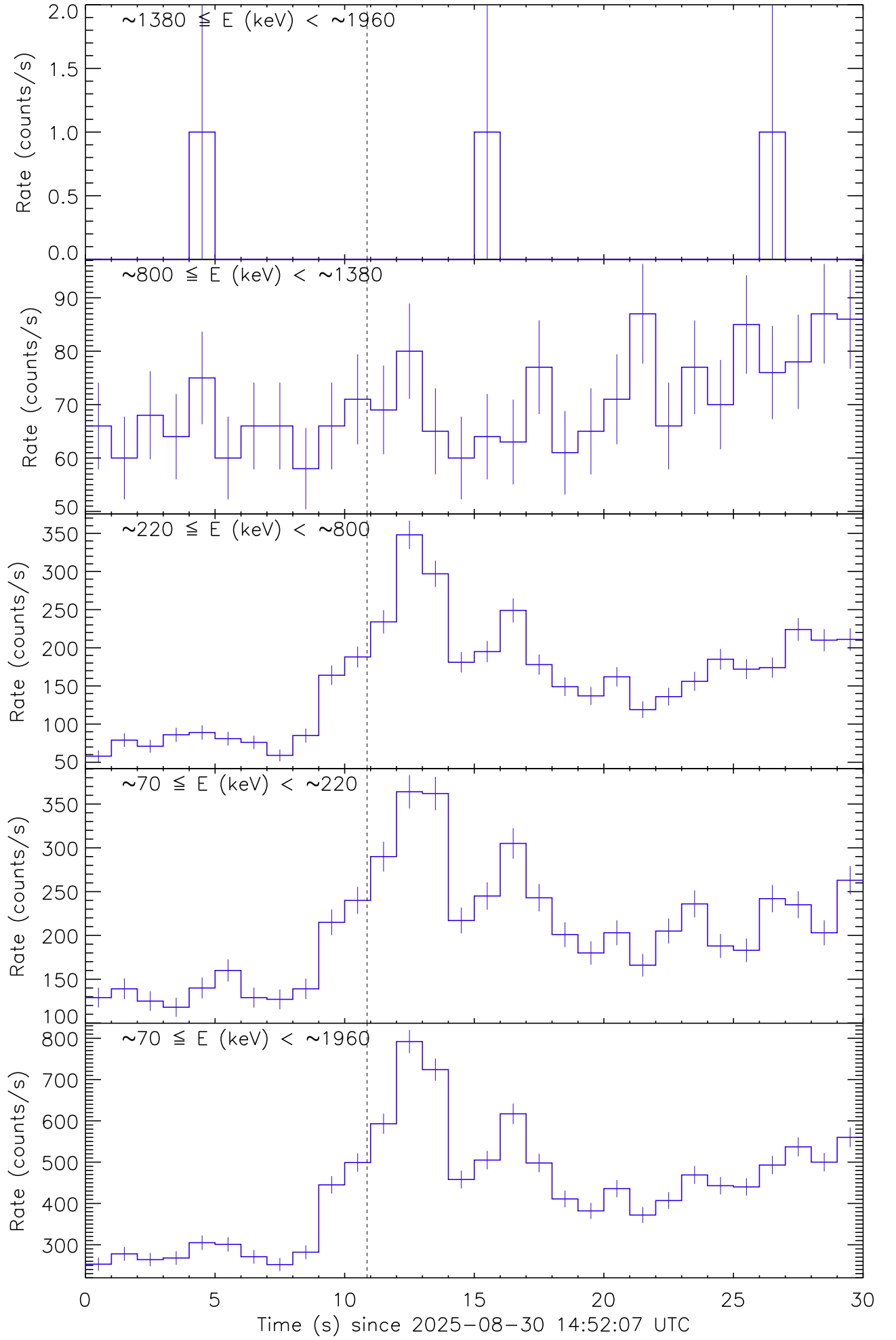
Figure 1: Raw count rate curves of GRB 250830C recorded by the detector unit no. 0. The vertical dashed line marks the trigger time by Konus-Wind.
