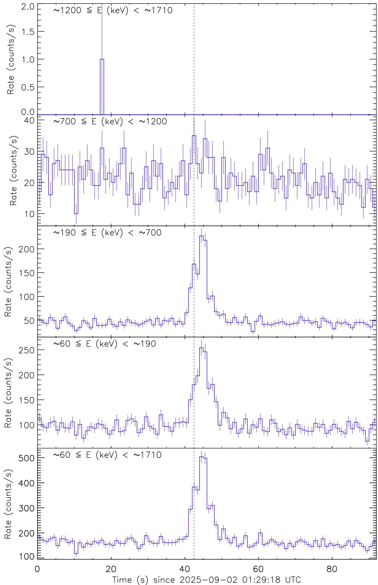
Figure 1: Raw count rate curves of GRB 250902A recorded by the detector unit no. 1. The vertical dashed line marks the trigger time by Fermi/GBM.
