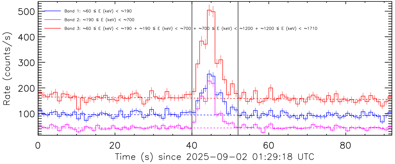
Figure 2: Background fit to the data from the detector unit no.1 by a linear function. Pre-burst and post-burst intervals which were used for the background fit are delimited by the vertical solid lines.
