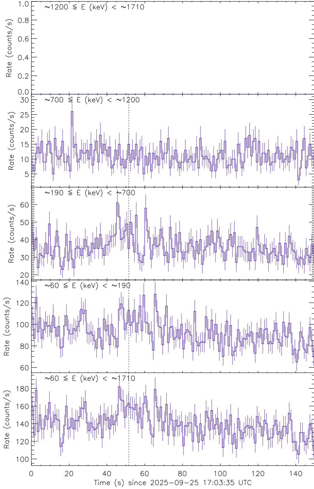
Figure 1: Raw count rate curves of GRB 250925A recorded by the detector unit no. 1. The vertical dashed line marks the trigger time by Swift/BAT.
