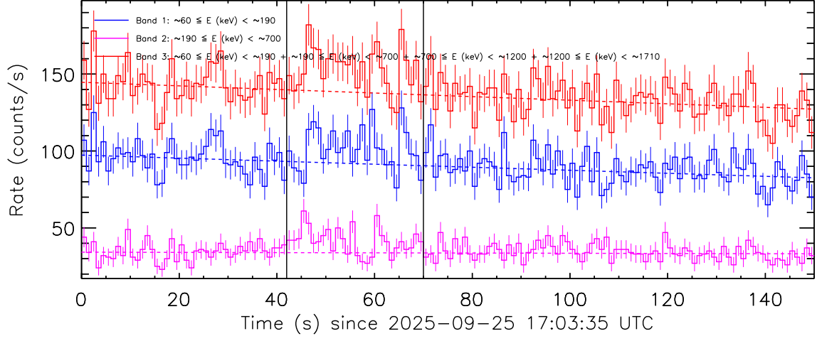
Figure 2: Background fit to the data from the detector unit no. 1 by a linear function. The pre-burst and post-burst intervals which were used for the background fit are delimited by the vertical solid lines.
