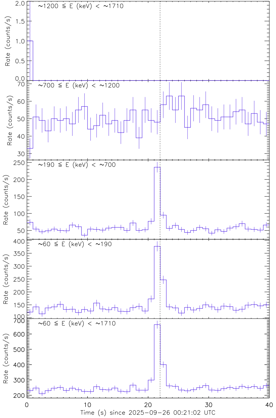
Figure 4: Raw count rate curves of GRB 250926A recorded by the detector unit no. 1. The vertical dashed line marks the trigger time by Fermi/GBM.
