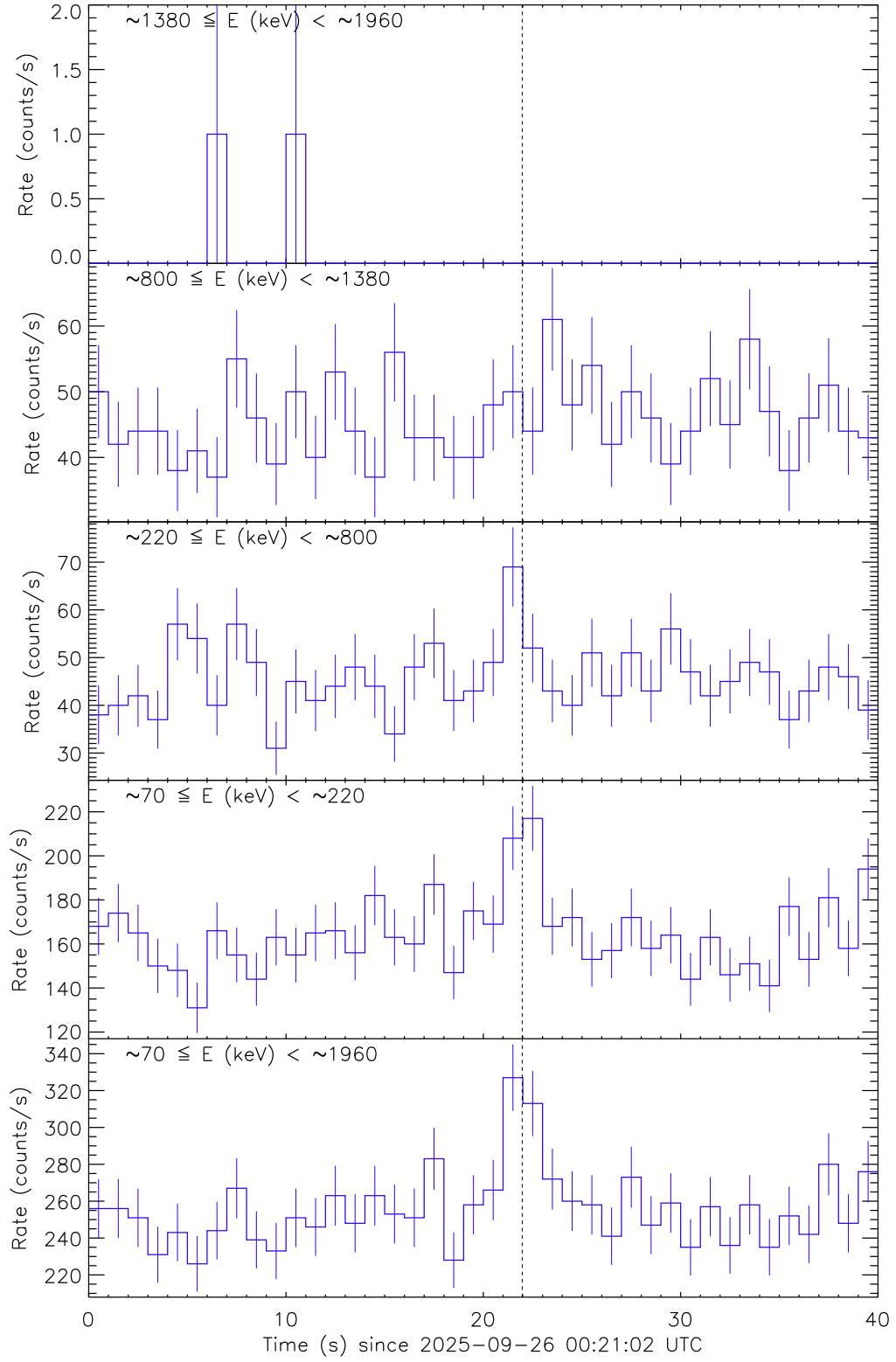
Figure 1: Raw count rate curves of GRB 250926A recorded by the detector unit no. 0. The vertical dashed line marks the trigger time by Fermi/GBM.
