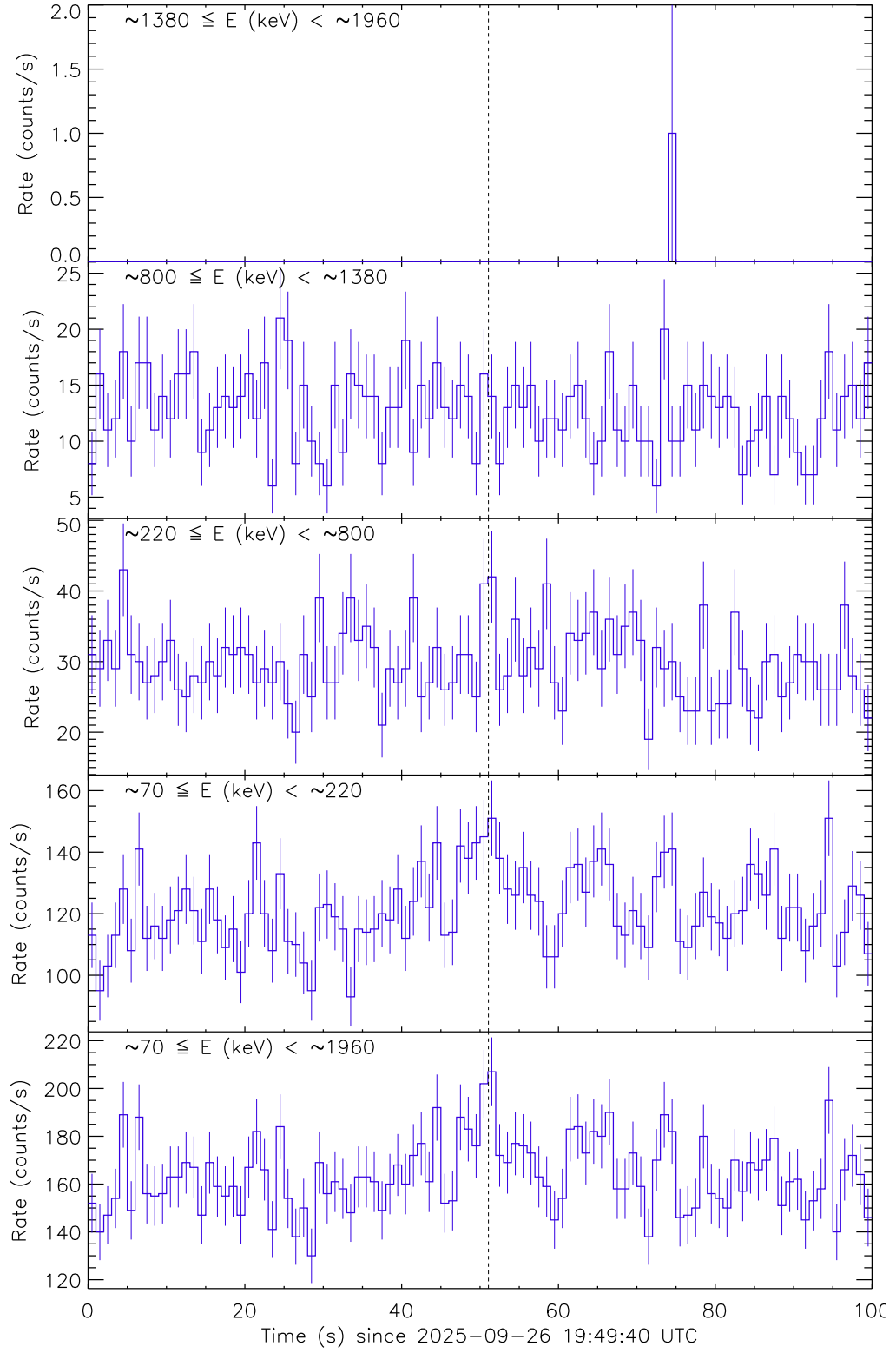
Figure 1: Raw count rate curves of GRB 250926B recorded by the detector unit no. 0. The vertical dashed line marks the trigger time by Fermi/GBM.
