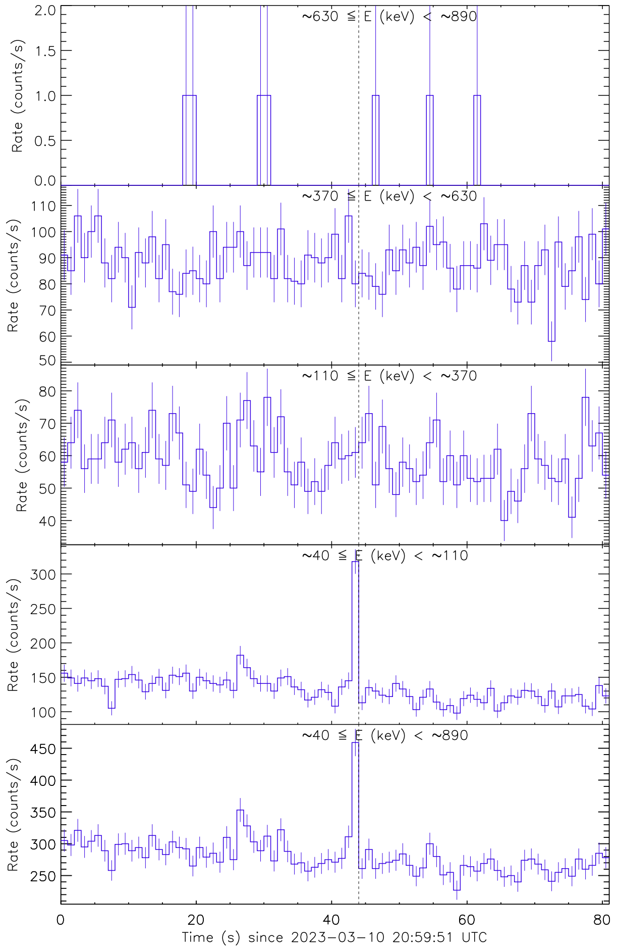
Figure 1: Raw count rate curves of SGR 1806-20 recorded by the detector unit no. 0. The vertical dashed line marks the trigger time by Swift/BAT.
