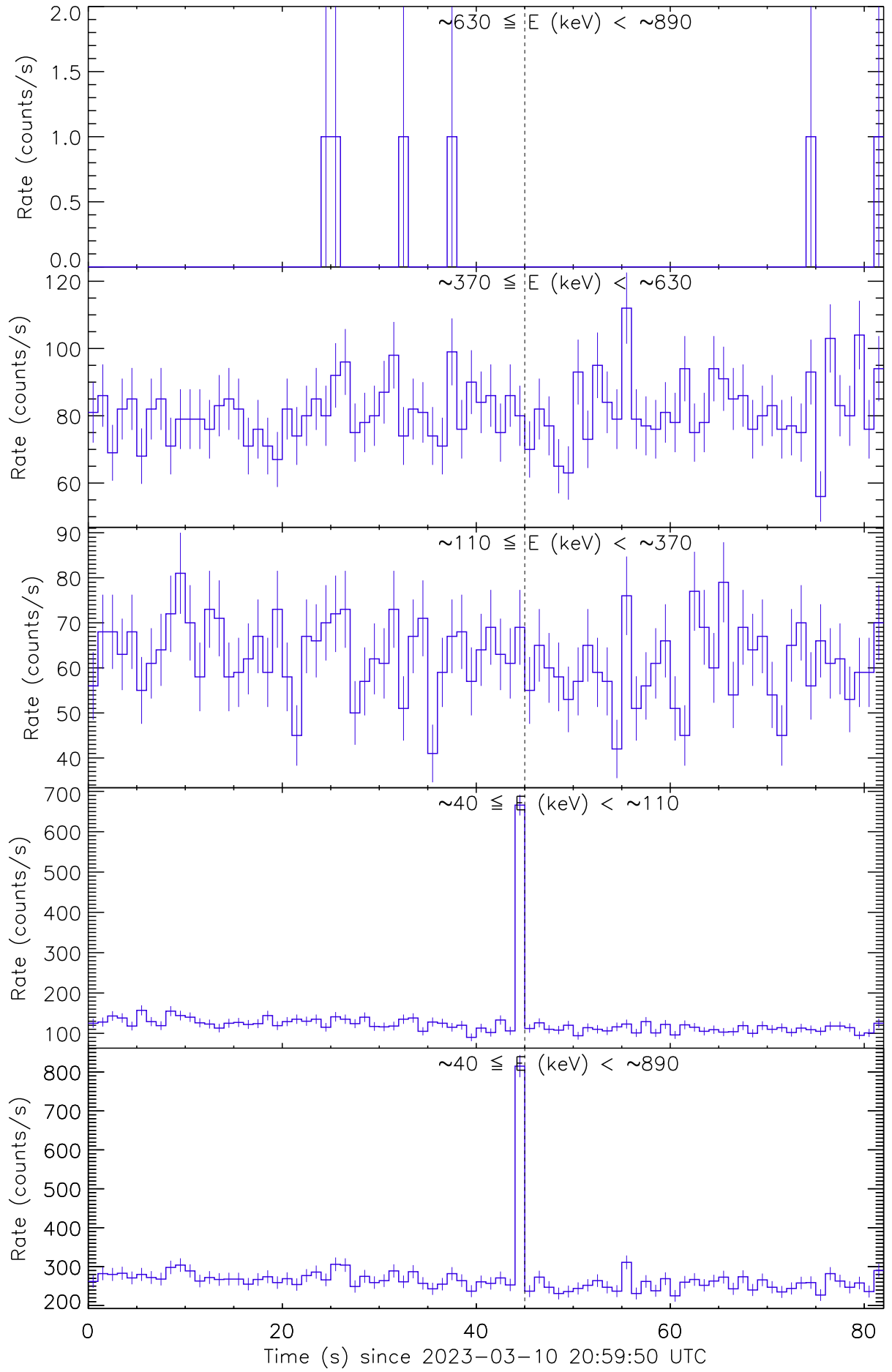
Figure 4: Raw count rate curves of SGR 1806-20 recorded by the detector unit no. 1. The vertical dashed line marks the trigger time by Swift/BAT.
