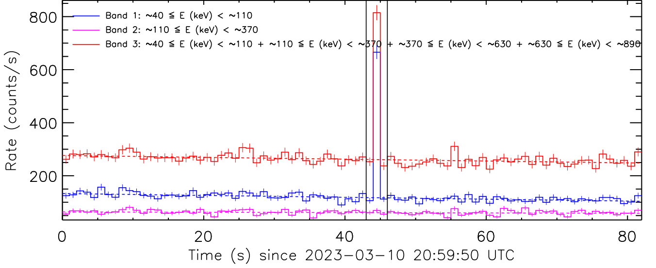
Figure 5: Background fit to the data from the detector unit no.1 by a linear function. The pre-burst and post-burst intervals which were used for the background fit are delimited by the vertical solid lines.
